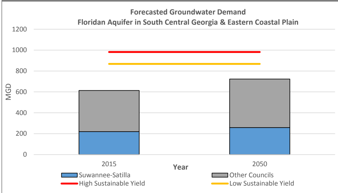
Figure 5-1: Floridan Aquifer Demand vs. Estimated Yield
